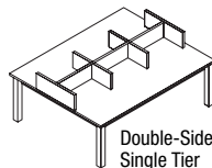
Square GLRT
